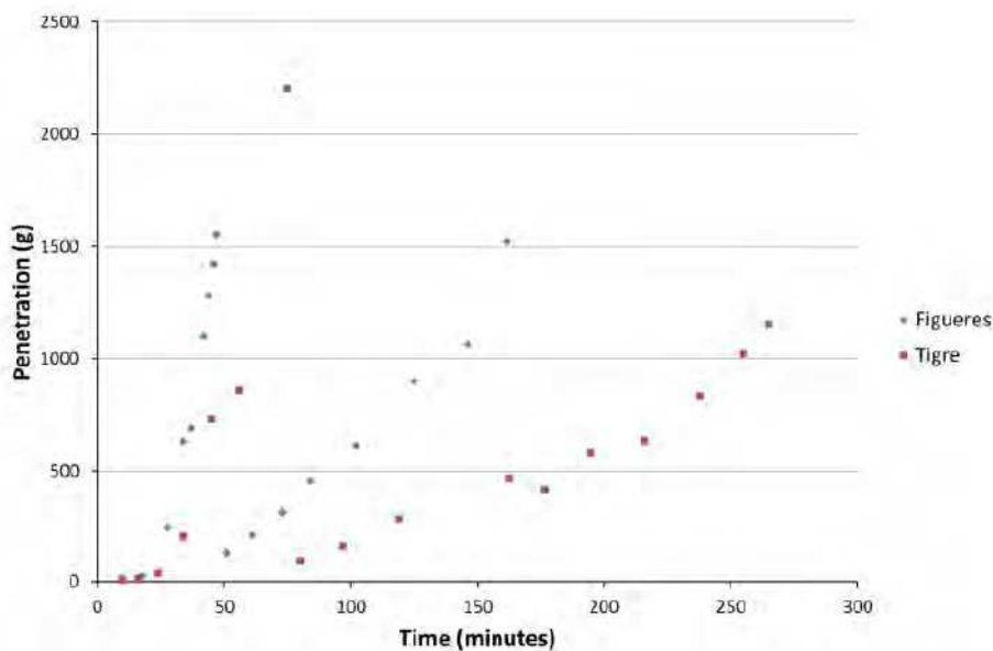
Figure 10. Raw data from Workable Life test for Figueres (15 %/30 min) and Tigre (10 %/30 min).
