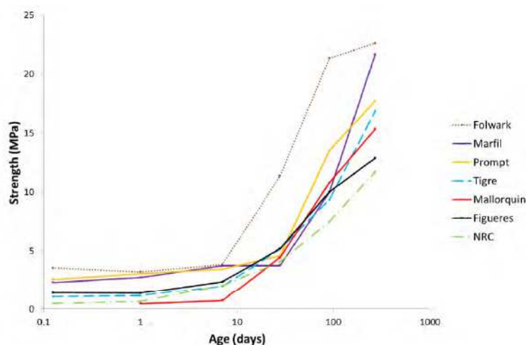
Figure 5. Compressive strength development of mortars produced at w/c = 0.6 .
