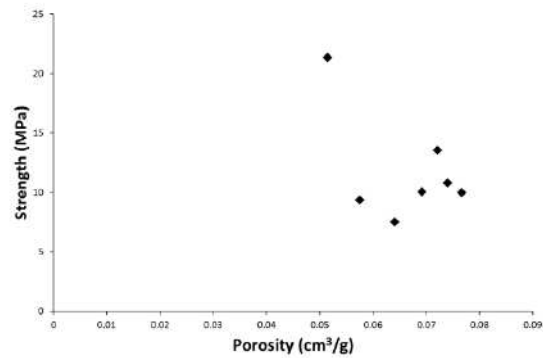
Figure 7. Strength – porosity >0.03 \mu\text{m} relationships of ROCEM mortars.
