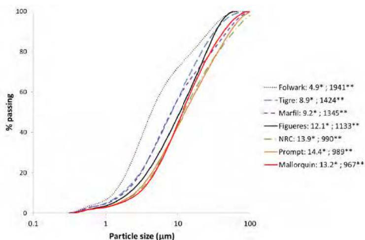
Figure 2. Particle size distribution * D_{50} (mm); ** Specific surface area ( \text{m}^2/\text{kg} )
