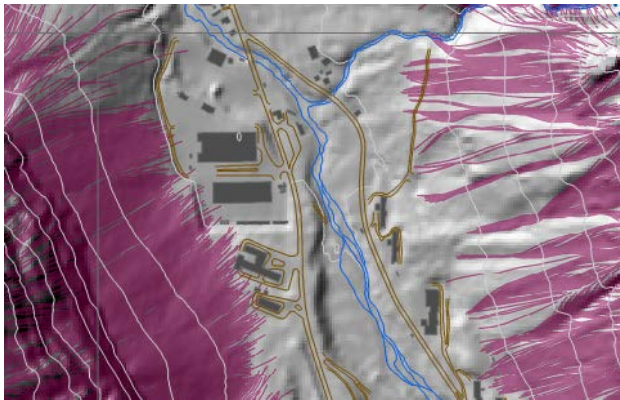
Figure 5: Rock fall endangered area with trajectories of a 100 years scenario (block size approx. 3 m 3 ) derived from ROF-MOD 3D.
