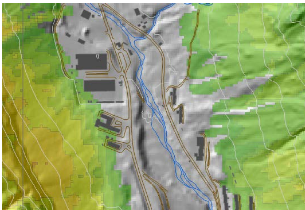
Figure 6: Rock fall endangered area with energies of a 100 years scenario (block size approx. 3 m 3 ) derived from ROF-MOD 3D.
