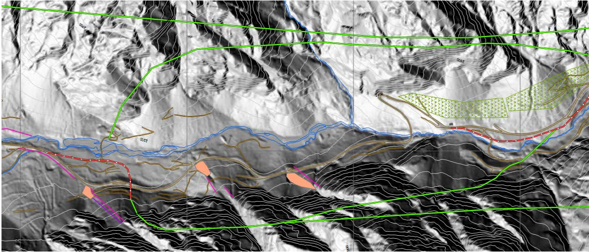
Figure 9: Area along the analysed valley with different possible protection measures like tunnels (green), road relocations (red), retention basins for debris flows (orange) and deflection dams (violet).
