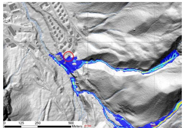
Figure 8: Debris flow affected area with one element at risk (red circle). This object can be selected automatically in a GIS when cutting the element with the process layer.
