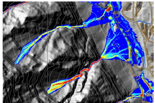
Figure 7: Process areas with indication of flow heights of debris flows derived from the model RAMMS.
