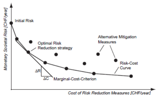
Figure 4: Risk-cost diagram which illustrates the optimisation of mitigation measures by using the marginal-cost-criterion. Where the tangent touches the risk-cost curve the economical optimised combination of measures under the given assumptions is suggested (Bründl et al., 2009b).
